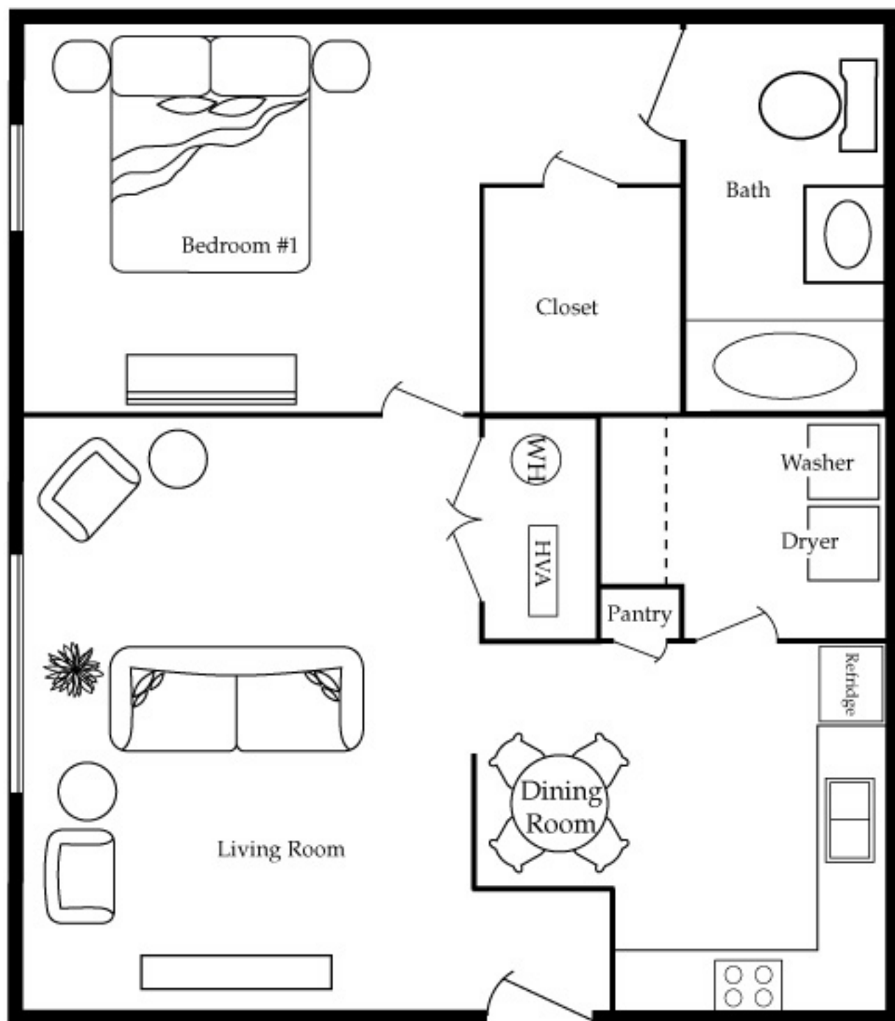
1 Bedroom, Model B 598 sf
